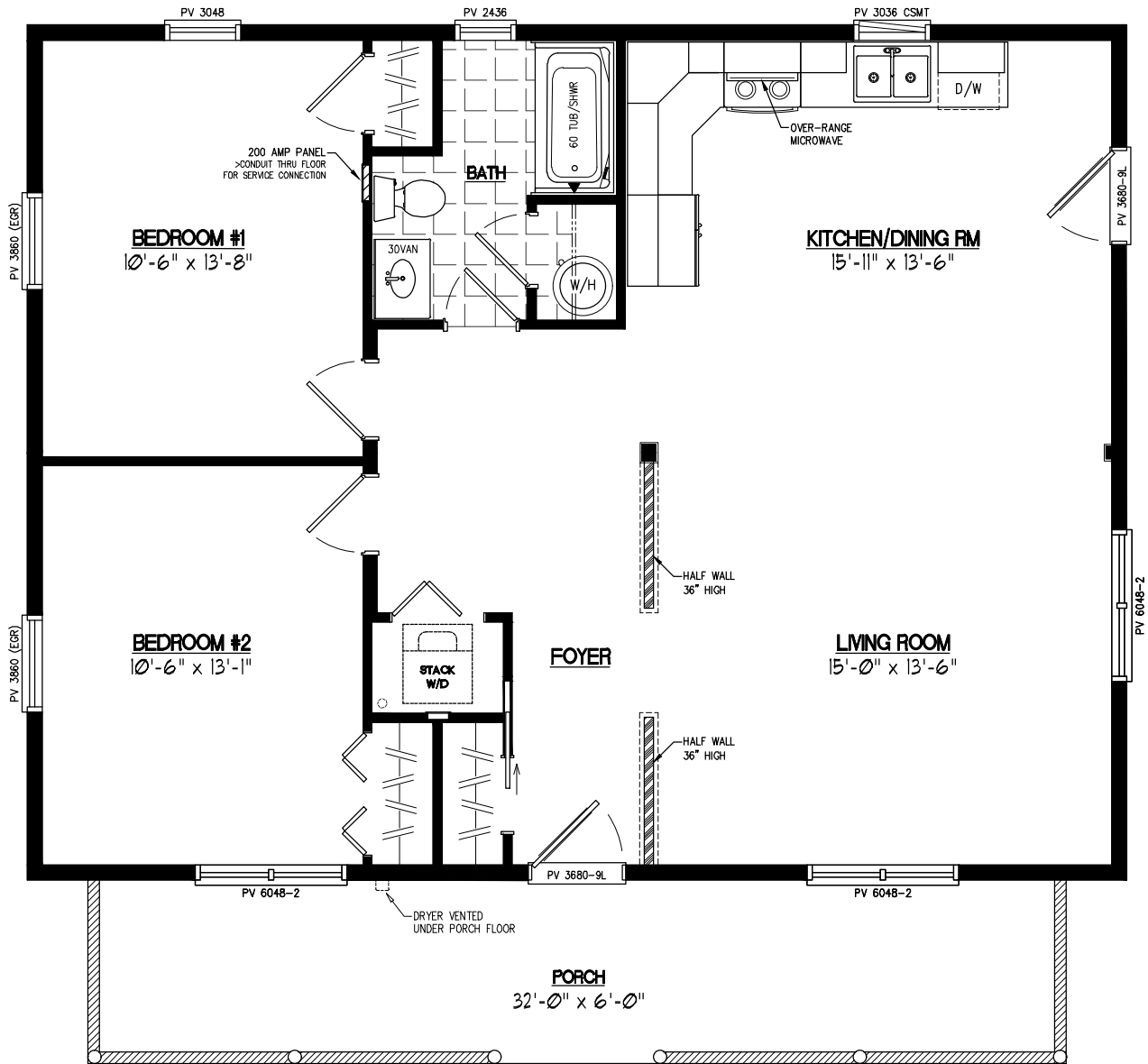
28x36 MUSKETEER Plan #28MK1502
