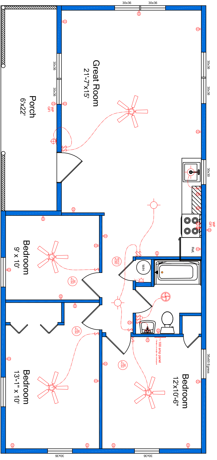
Plan 22CC603-H 22'x48' with 6' x 22' porch included
