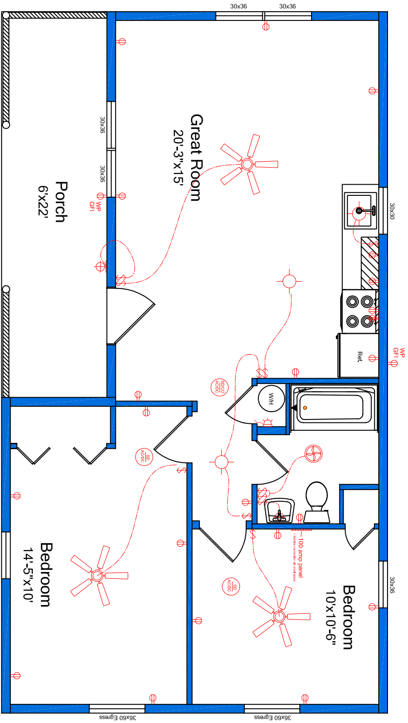
Plan 22CC602-H 22'x40' with 6' x 22' porch included
