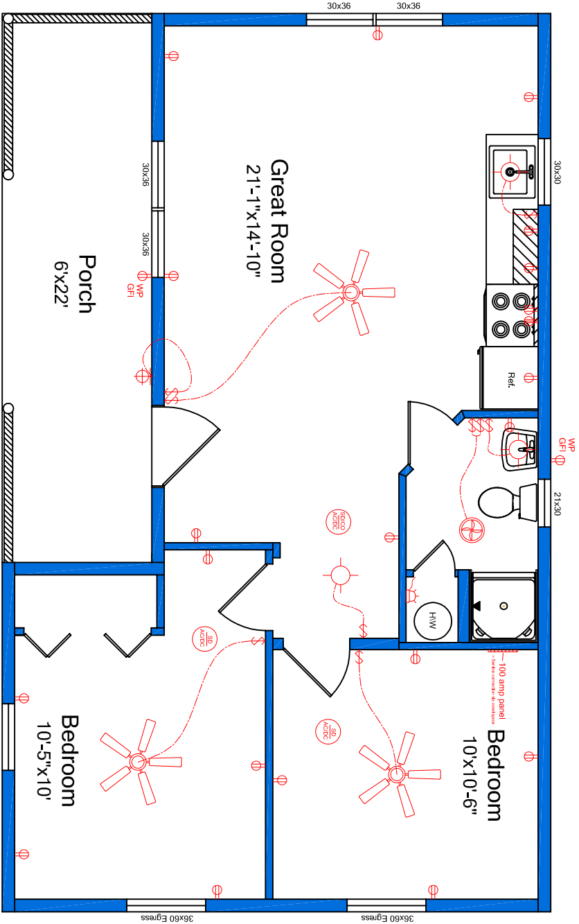
Plan 22CC601-H 22'x36' with 6' x 22' porch included
