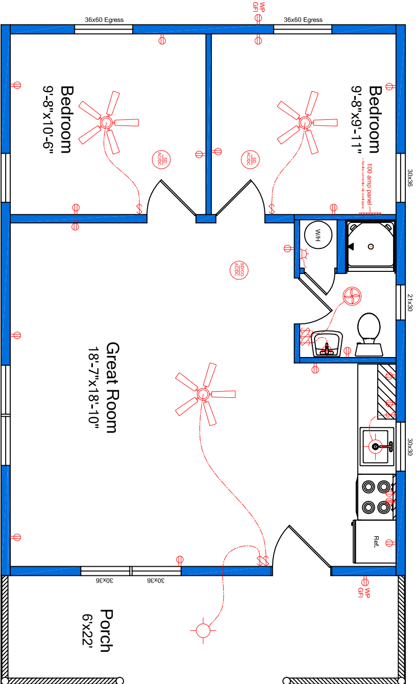
Plan 22CC501-H 22'x36' with 6' porch included
